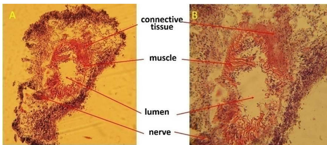
Figure17. Histology of tube feet. A. 4X magnification, B. 40X magnification.
